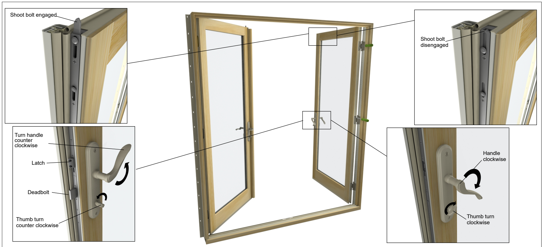
Figure 10 Turn handle and thumb turn counterclockwise to lock; clockwise to unlock.
