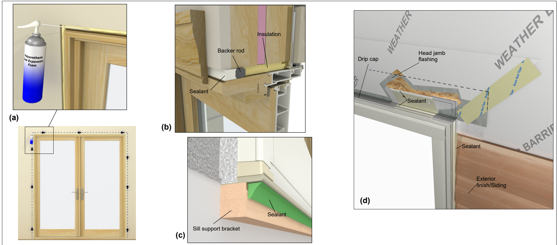
Figure 9 Sealing the installation.
