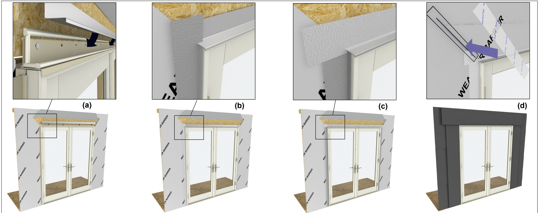
Figure 8 Flashing the Installation
