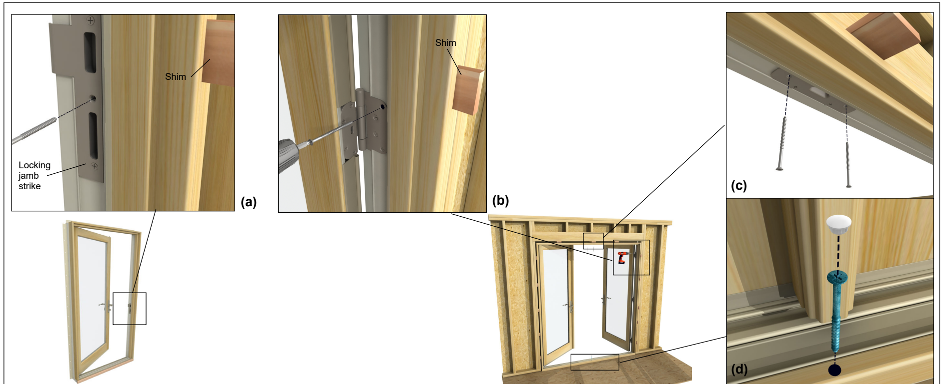
Figure 6 Additional Fastening
