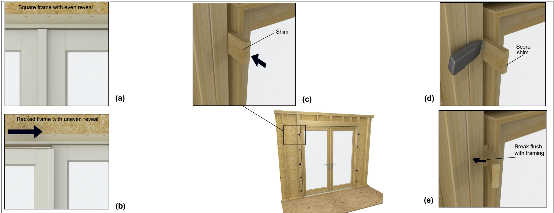
Figure 7 Final adjustments
