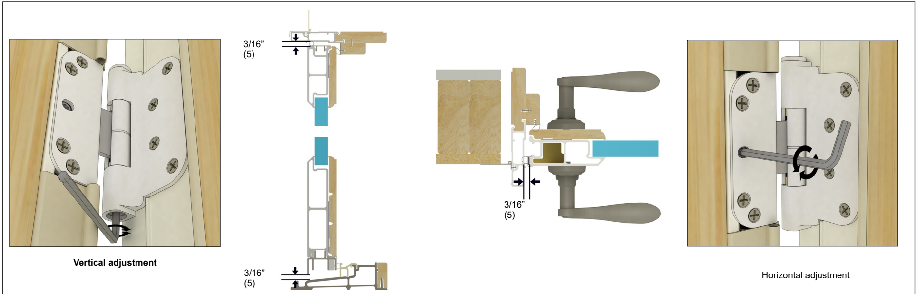
Figure 11 Hinge adjustment
