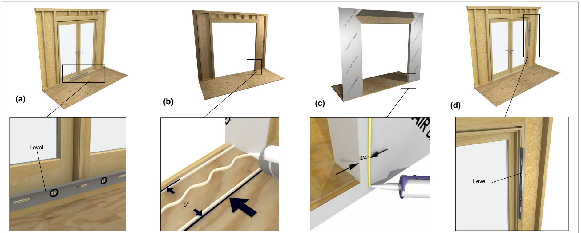
Figure 4 Preparing the unit for installation.
